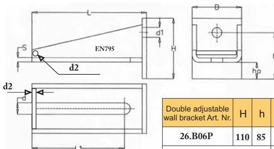
Double adjustable wall bracket
